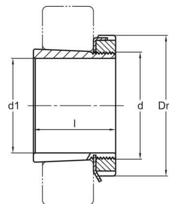
ADAPTER SLEEVES H
