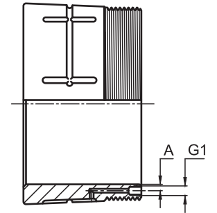
REPRESENTATION OF THE OIL GROOVES FOR HYDRAULIC SLEEVES OHE ...H, OHA ...H, OHS ...H
