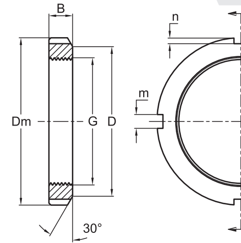
NUTS KM, KML
