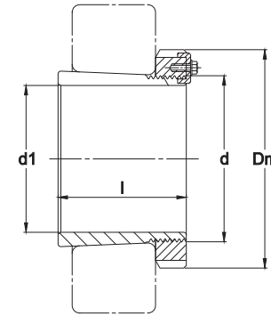
ADAPTER SLEEVES H WITH HM/MS
